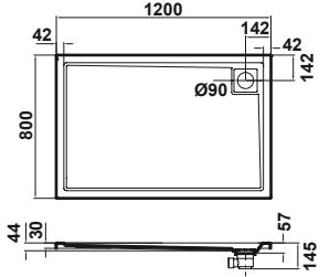
PLATO RECTANGULAR 120x80 / 100x70 120x80 / 100x70 ANGULAR SHOWER TRAY
