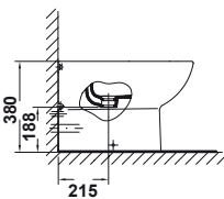
TAPA BIDÉ # 51630 BIDET COVER
