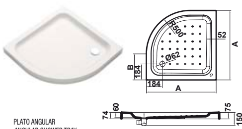
PLATO ANGULAR ANGULAR SHOWER TRAY
