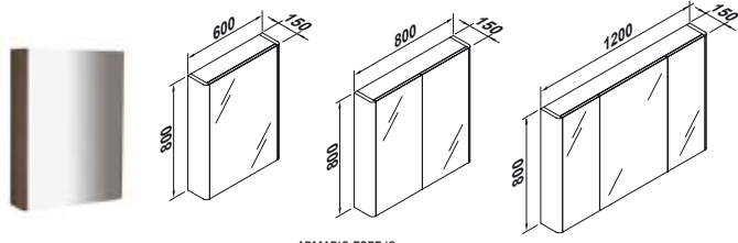
ARMARIO ESPEJO MIRROR CABINET
