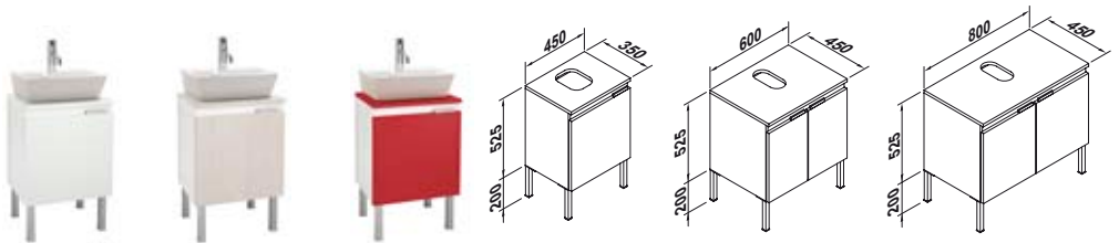
MUEBLE BASE LAVABO 45 x 35 / 60 x 45 / 80 x 45 cm. 45 x 35 / 60 x 45 / 80 x 45 cm. VANITY UNIT
